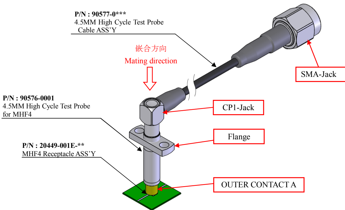
Figure.1 parts names
