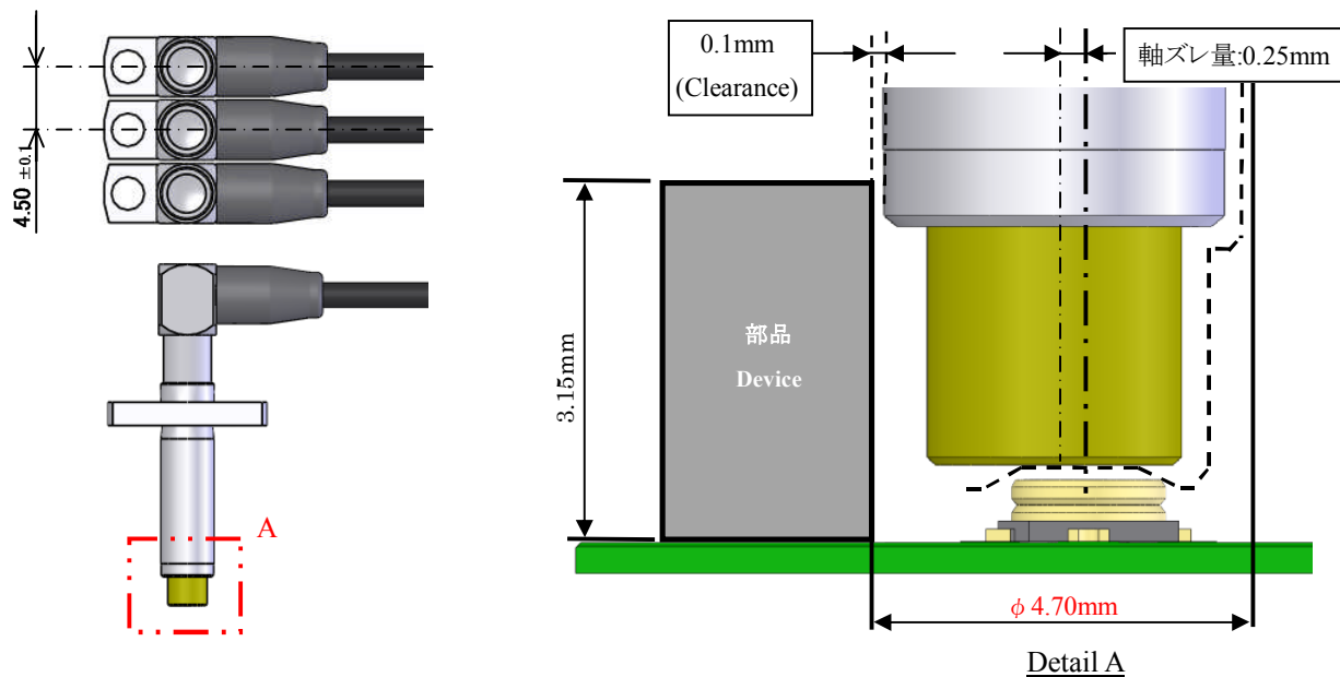
Figure.4 部品配置禁止区域 Device placement prohibited area
