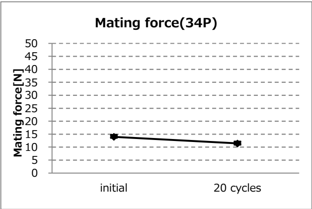
Graph-15. A change of mating force (34P)
