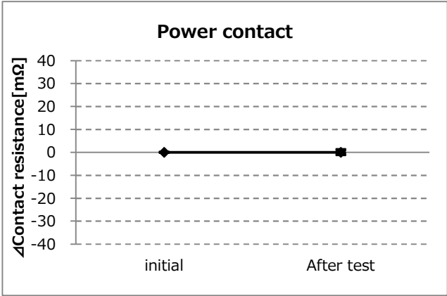
Graph-32. A change of power contact resistance
