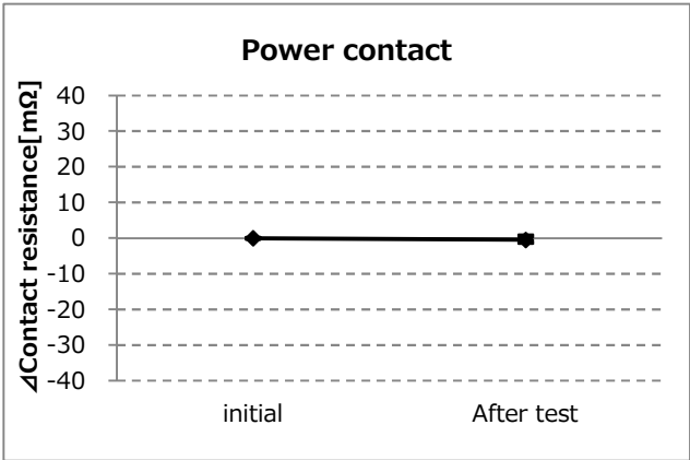
Graph-30. A change of power contact resistance
