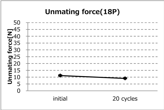
Graph-8. A change of unmating force (18P)
