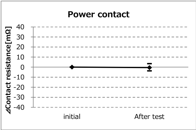
Graph-36. A change of power contact resistance
