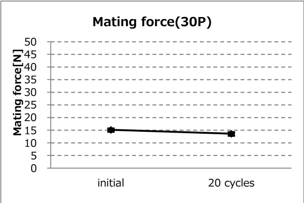
Graph-13. A change of mating force (30P)
