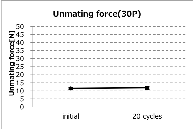
Graph-14. A change of unmating force (30P)
