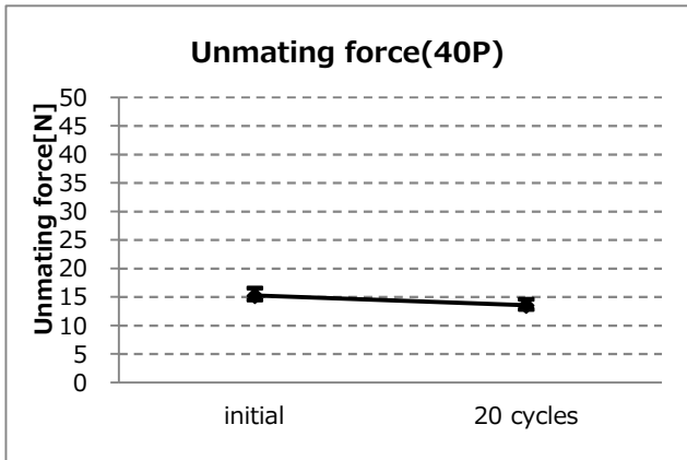
Graph-18. A change of unmating force (40P)
