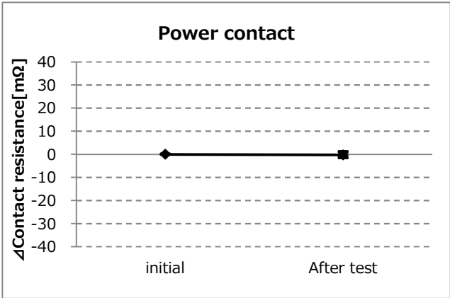
Graph-34. A change of power contact resistance
