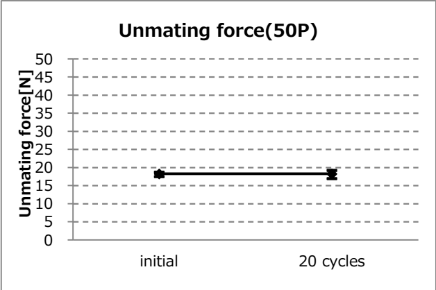
Graph-20. A change of unmating force (50P)
