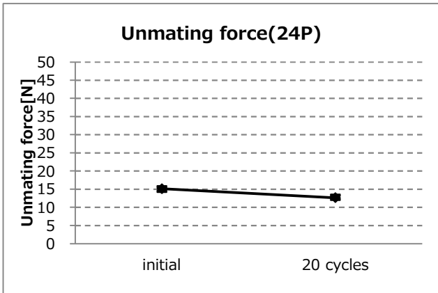
Graph-12. A change of unmating force (24P)
