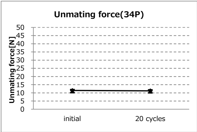
Graph-16. A change of unmating force (34P)
