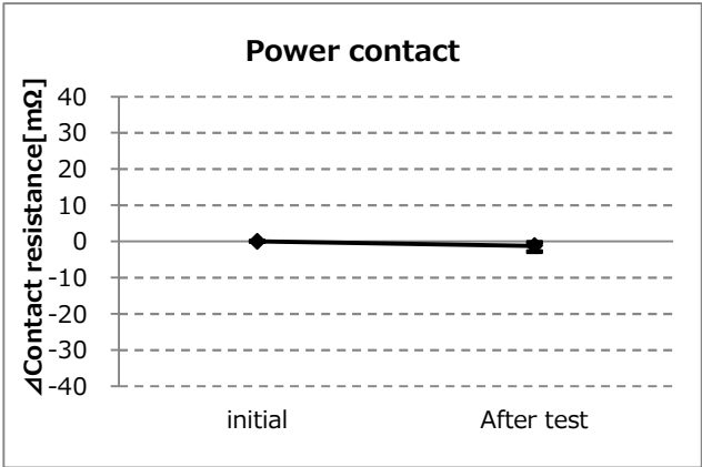
Graph-28. A change of power contact resistance
