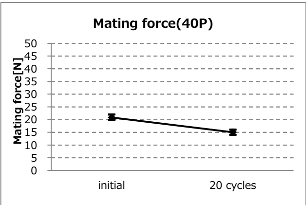
Graph-17. A change of mating force (40P)
