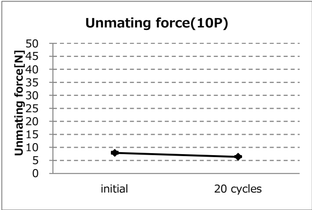
Graph-4. A change of unmating force (10P)
