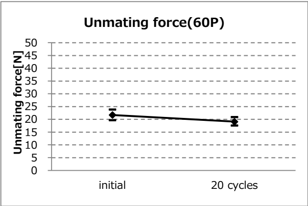
Graph-22. A change of unmating force (60P)
