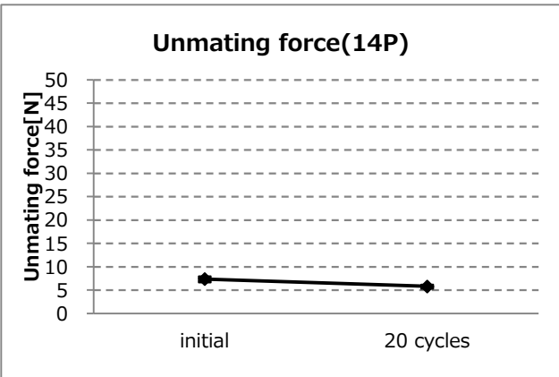
Graph-6. A change of unmating force (14P)
