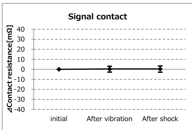
Graph-23. A change of signal contact resistance
