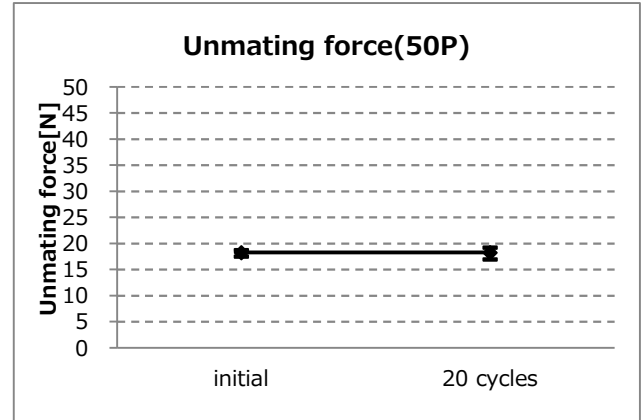
Graph-20. A change of unmatting force (50P)
