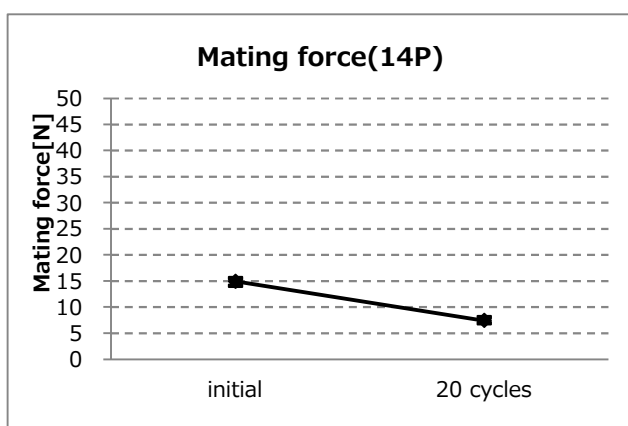
Graph-5. A change of mating force (14P)
