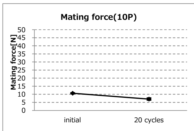
Graph-3. A change of mating force (10P)
