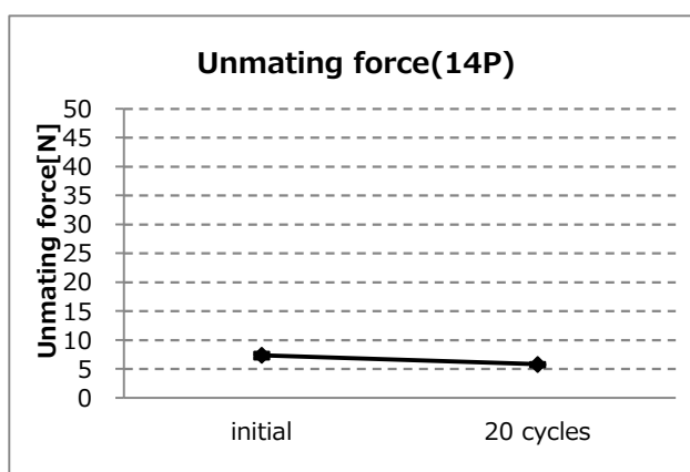
Graph-6. A change of unmating force (14P)
