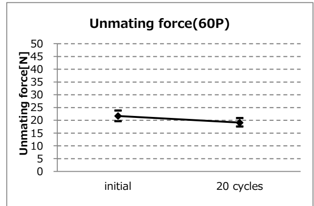
Graph-22. A change of unmatting force (60P)
