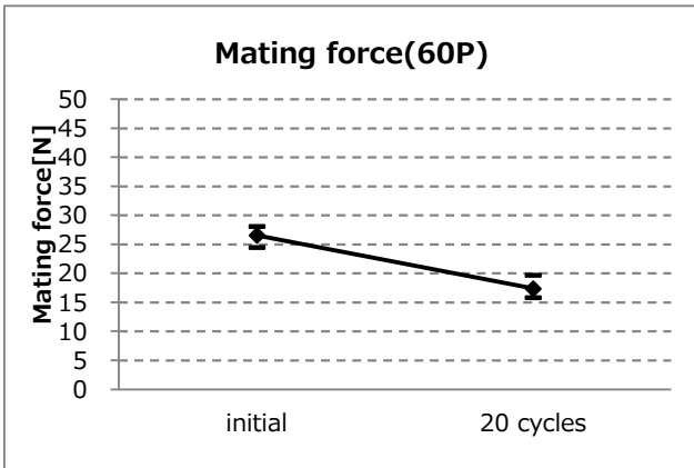
Graph-21. A change of mating force (60P)
