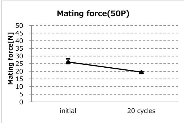
Graph-19. A change of mating force (50P)
