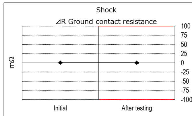
(Graph 10) Shock \Delta R Ground contact resistance
