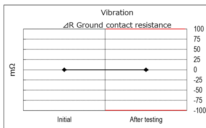
(Graph 8) Vibration ΔR Ground contact resistance
