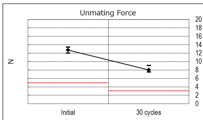
(Graph 3) Unmating Force
