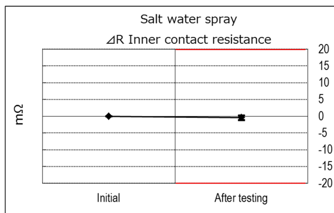
(Graph 15) Salt water spray \Delta R Inner contact resistance
