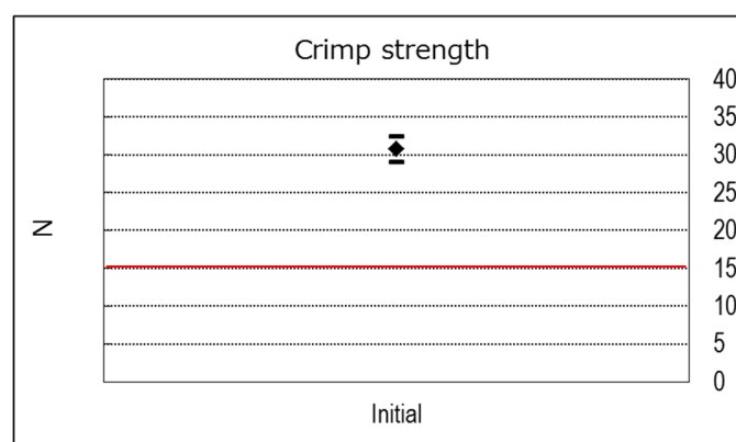
(Graph 4) Crimp strength
