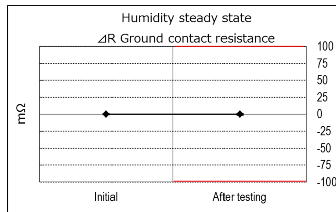
(Graph 14) Humidity steady state \Delta R Ground contact resistance
