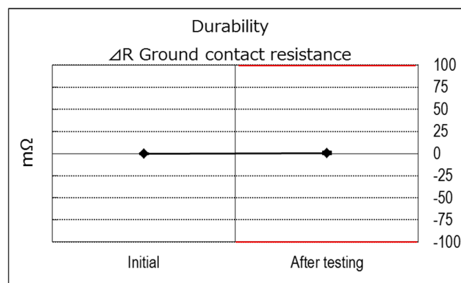
(Graph 6) Durability ΔR Ground contact resistance
