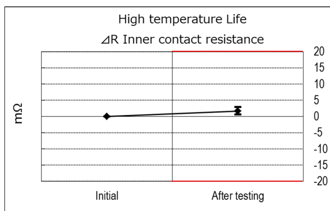
(Graph 17) High temperature life \Delta R Inner contact resistance
