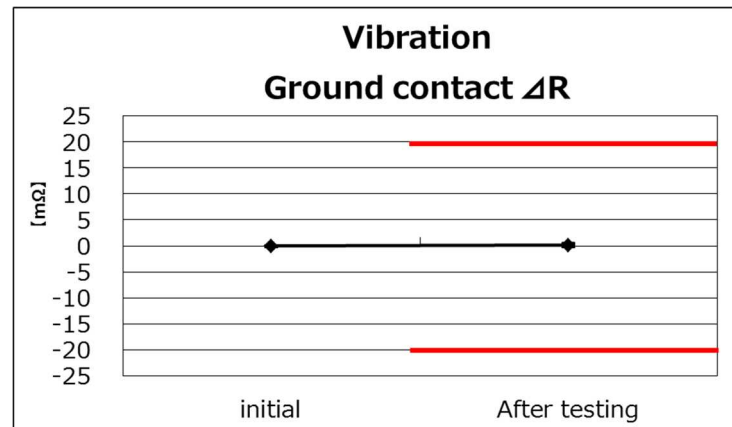
Graph 4. Group G Vibration
