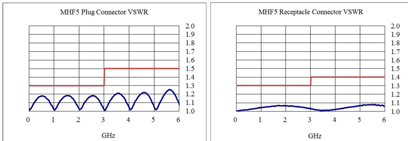
Graph 1 VSWR
