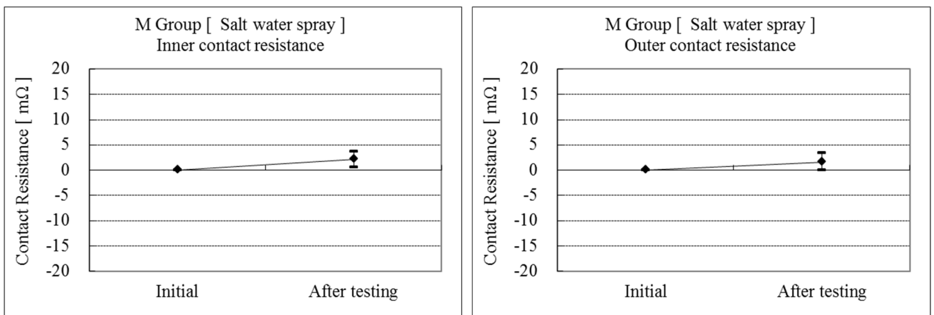
Graph 10 塩水噴霧
