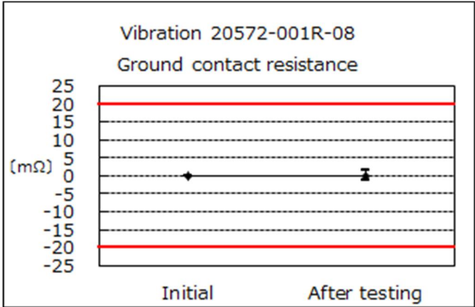
Graph 4 Vibration
