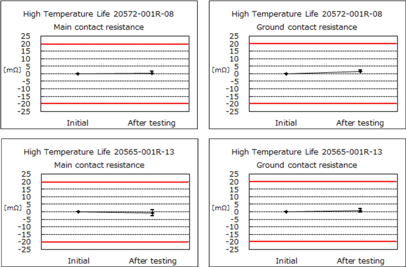
Graph 7 High temperature life
