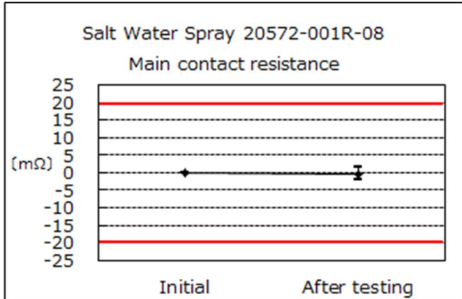
Graph 9 Salt Water Spray
