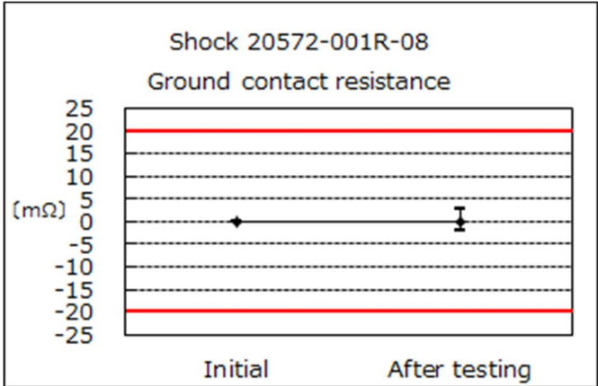
Graph 5 Shock
