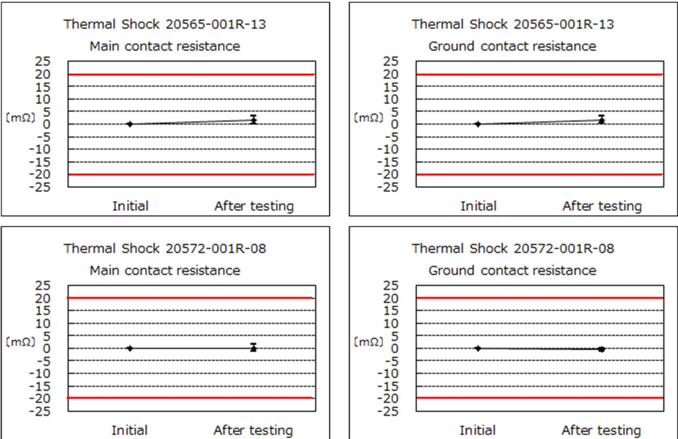
Graph 6 Thermal shock
