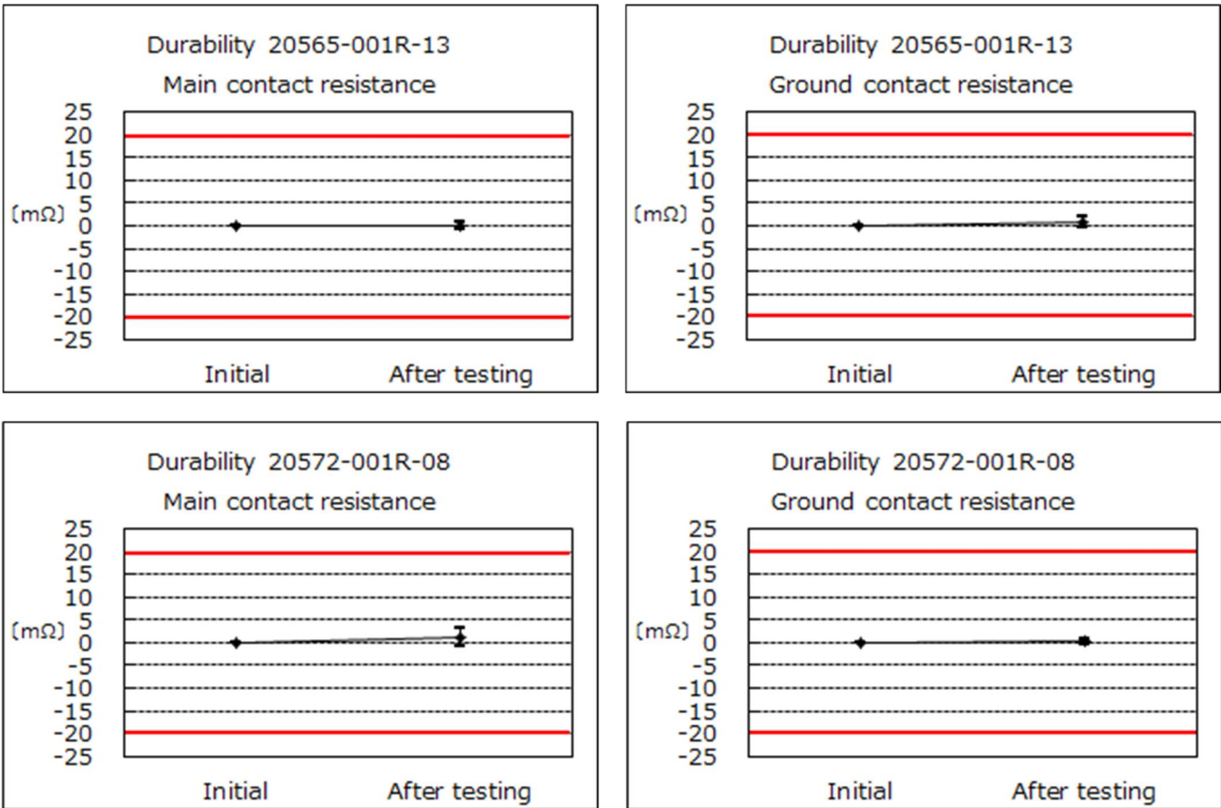
Graph 3 Durability
