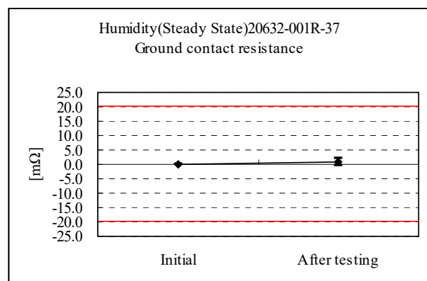
Graph 8 Humidity(Steady State)
