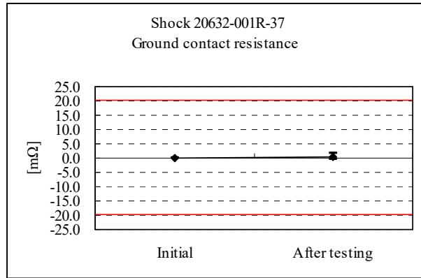
Graph 5 Shock
