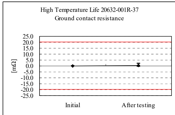
Graph 7 High Temperature
