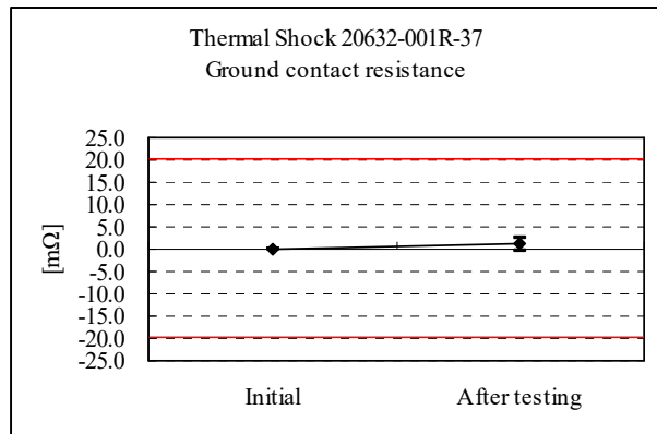
Graph 6 Thermal Shock
