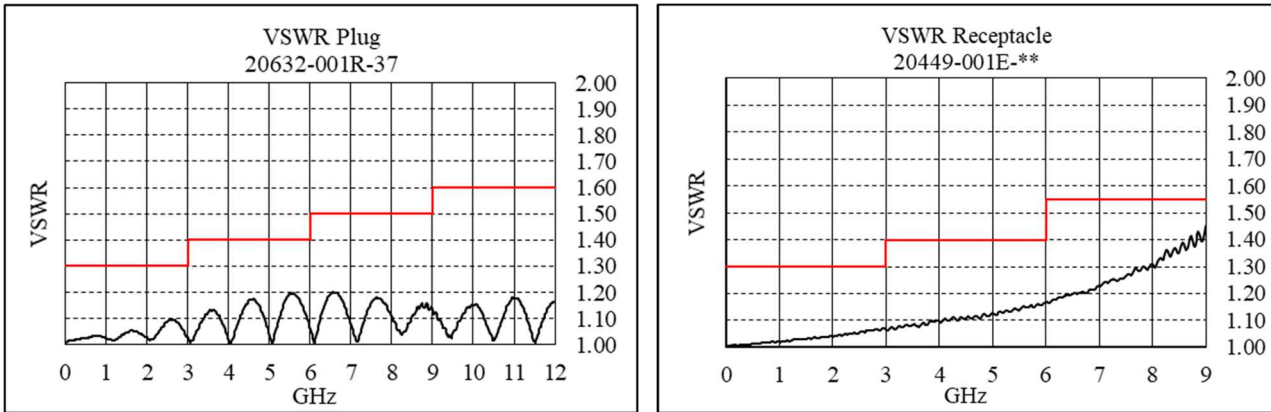
Graph 1 VSWR
