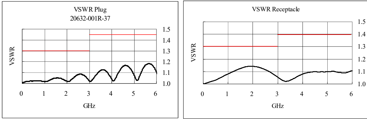
Graph 1 VSWR
