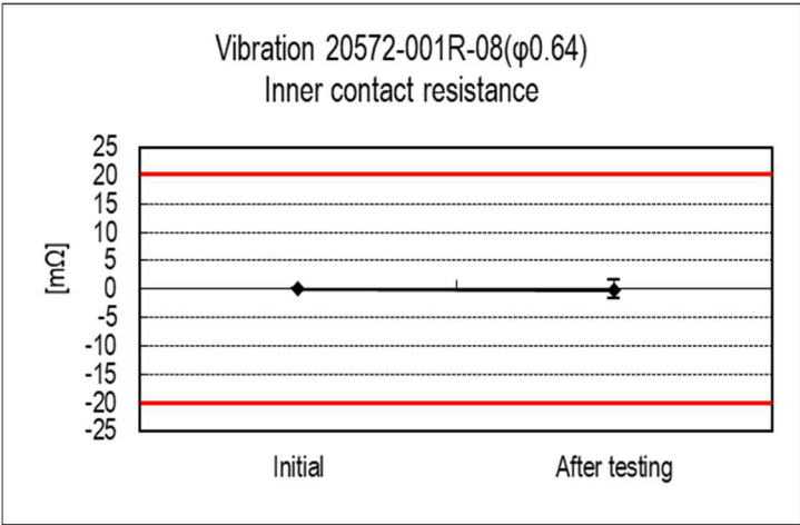
Graph 4 Vibration
