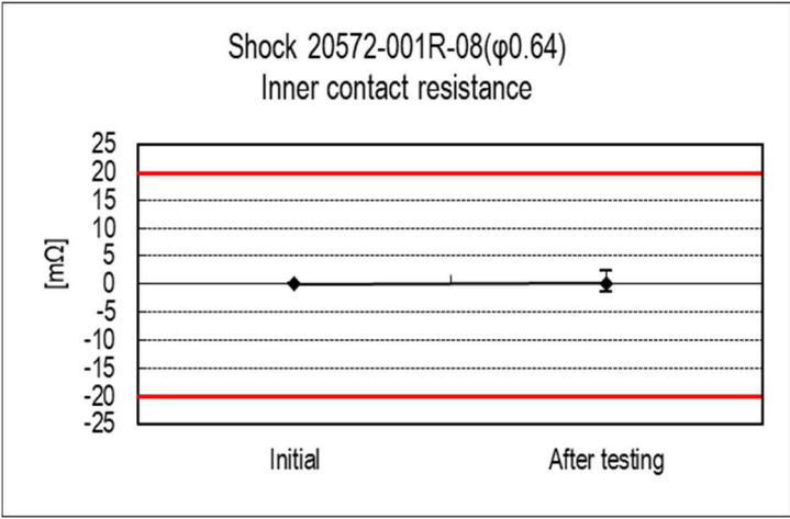
Graph 5 Shock
