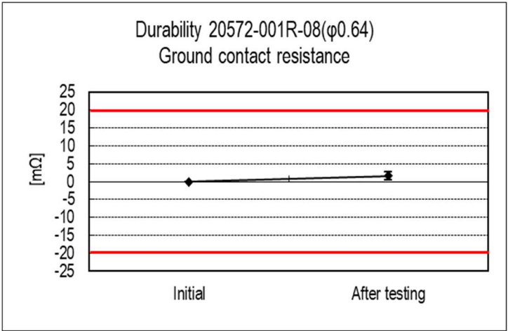
Graph 3 Durability
