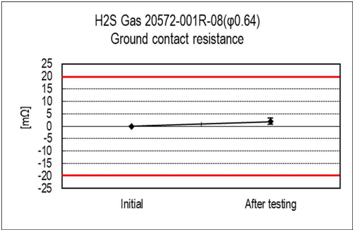
Graph 10 H2S Gas
