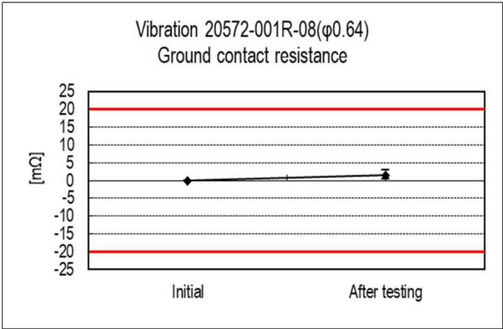
Graph 4 Vibration
