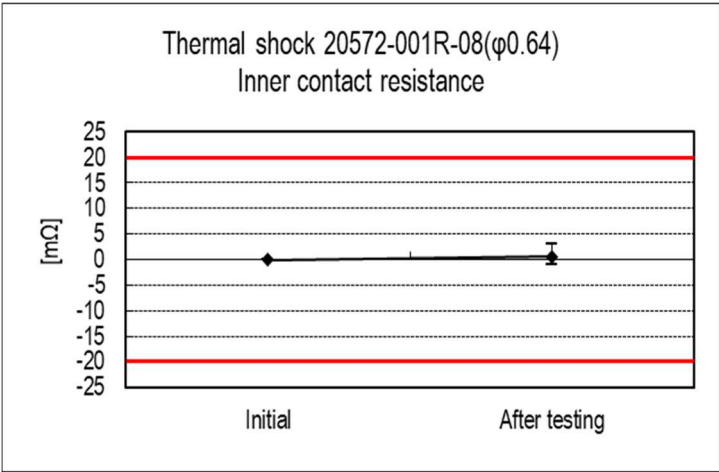
Graph 6 Thermal shock
