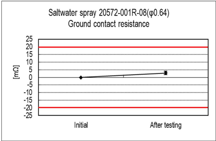
Graph 9 Saltwater spray
