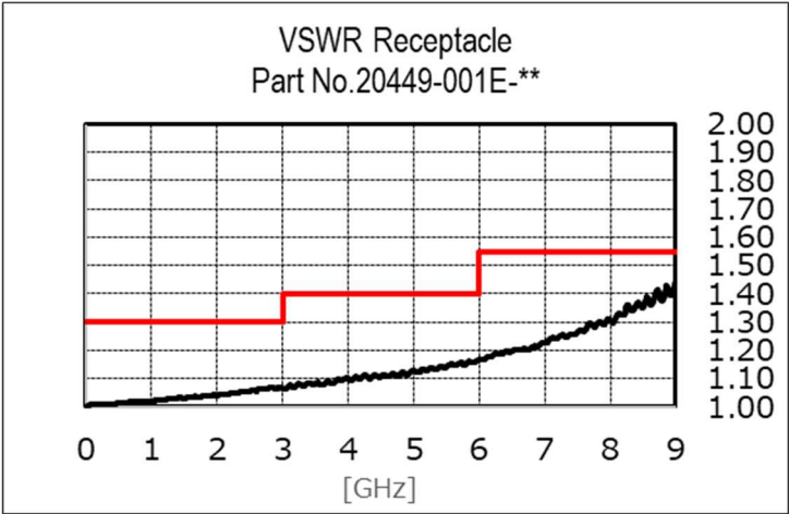
Graph 1 VSWR
