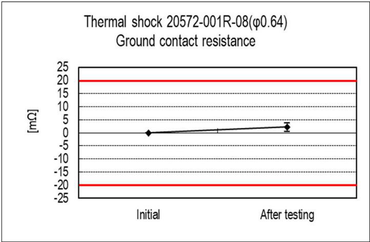
Graph 6 Thermal shock
