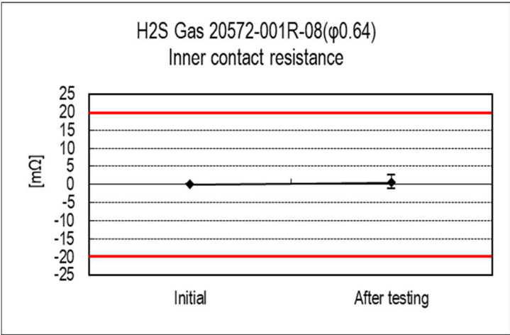
Graph 10 H2S Gas
