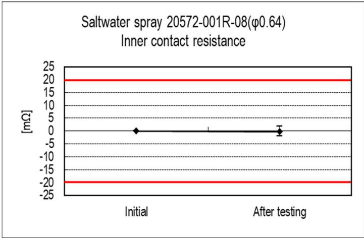
Graph 9 Saltwater spray
