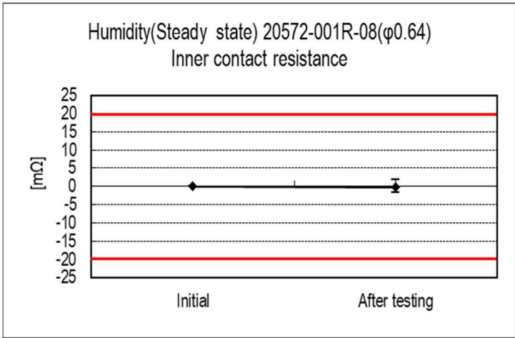
Graph 8 Humidity(Steady state)
