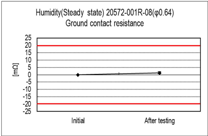
Graph 8 Humidity(Steady state)
