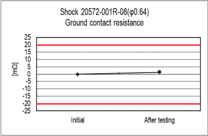
Graph 5 Shock
