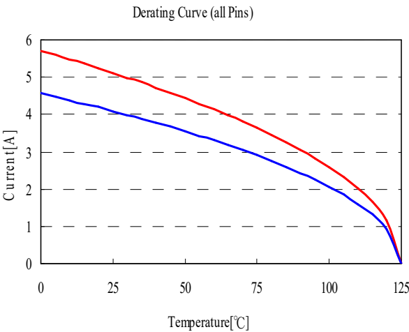
Graph 21. PG13 E13.2 Derating Curve
