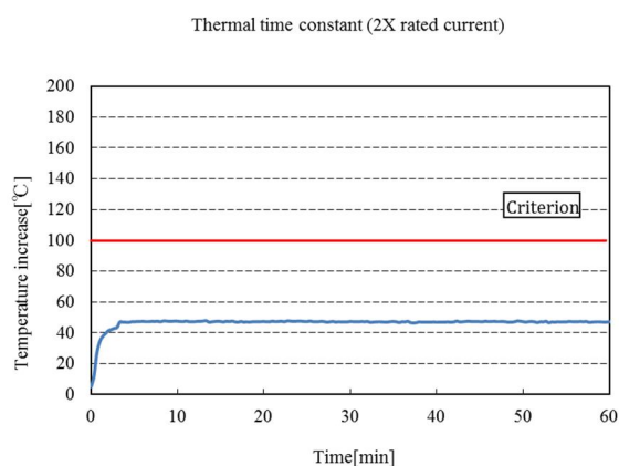
Graph 3. PG14 E14.1 Thermal time constant
