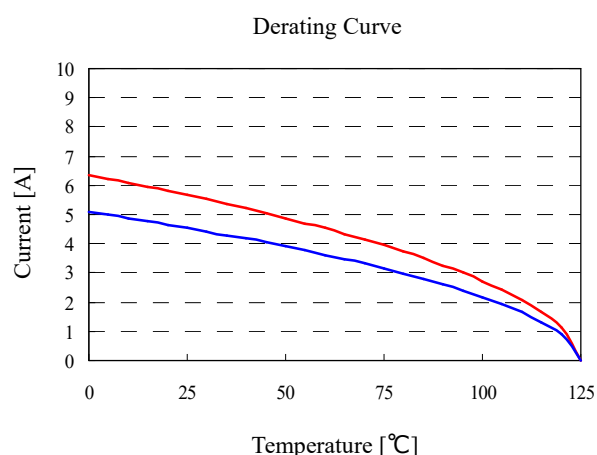
Graph 4. PG15 E12.2 Derating Curve
