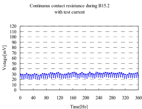
Graph 5. PG15 E14.0 Resistance Monitor
