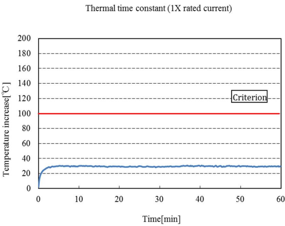
Graph 26. PG14 E14.1 Thermal time constant
