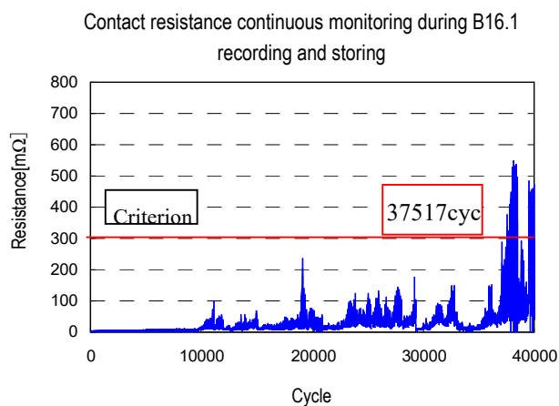
Graph 7. PG16 E16.0 Resistance Monitor
