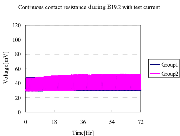
Graph 11. PG19 (E14.0) Resistance Monitor
