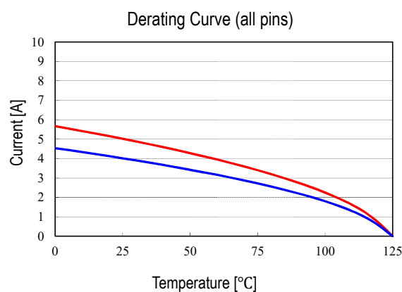
Graph 2. PG13 E13.2 Derating Curve with housing
