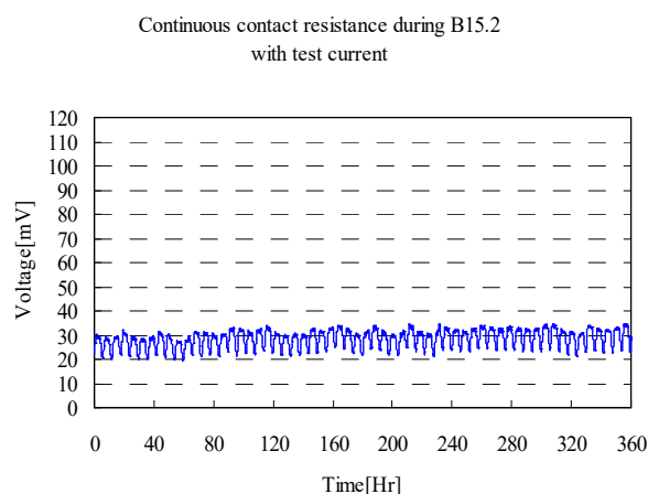
Graph 6. PG15 E14.0 Resistance Monitor
