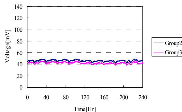
Graph 14. PG19 (E14.0) Resistance Monitor
