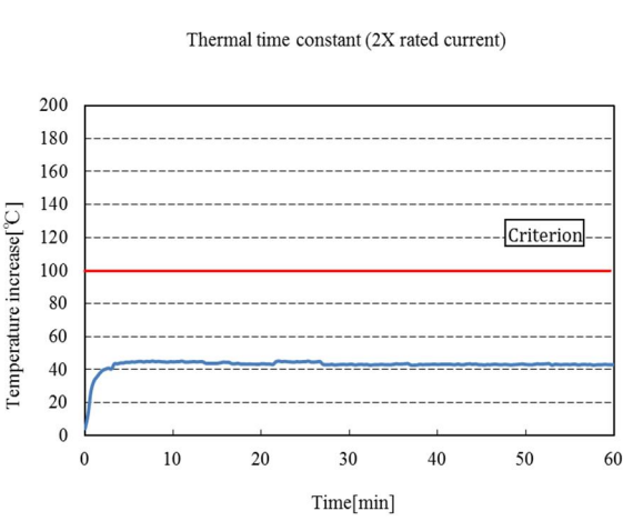
Graph 18. PG14 E14.1 Thermal time constant
