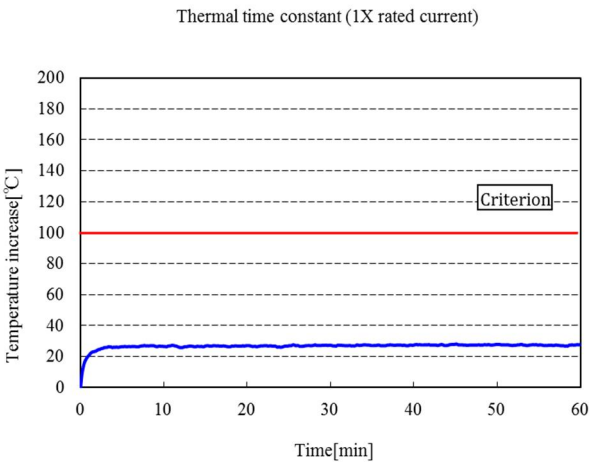
Graph 22. PG14 E14.1 Thermal time constant
