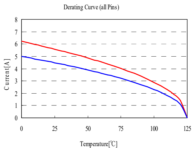
Graph 23. PG13 E13.2 Derating Curve
