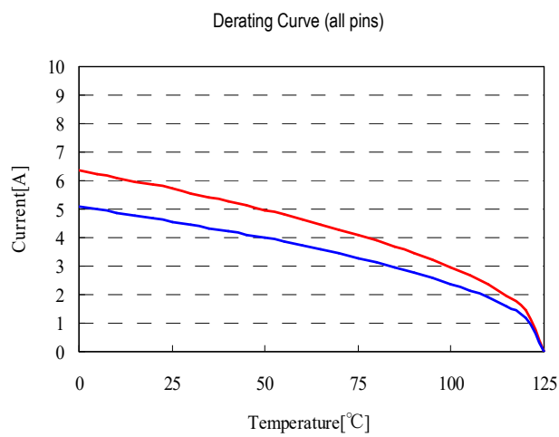
Graph 19. PG13 E13.2 Derating Curve
