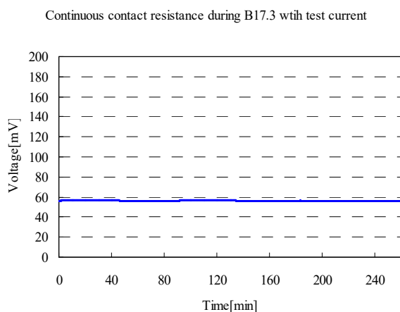
Graph 9. PG17 E14.0(B17.3) Resistance Monitor
