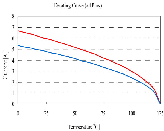
Graph 25. PG13 E13.2 Derating Curve
