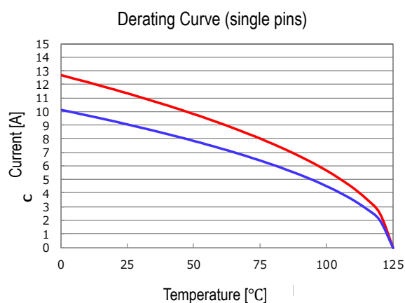
Graph 1. PG12 E12.1 Derating Curve without housing
