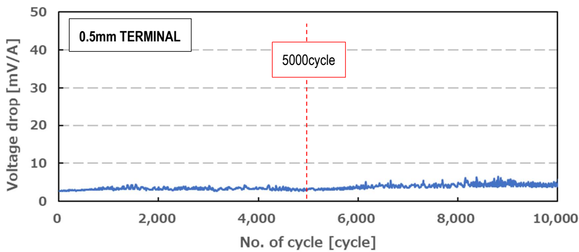
Graph 5. Monitoring result of 0.5mm terminal resistance for fretting corrosion
