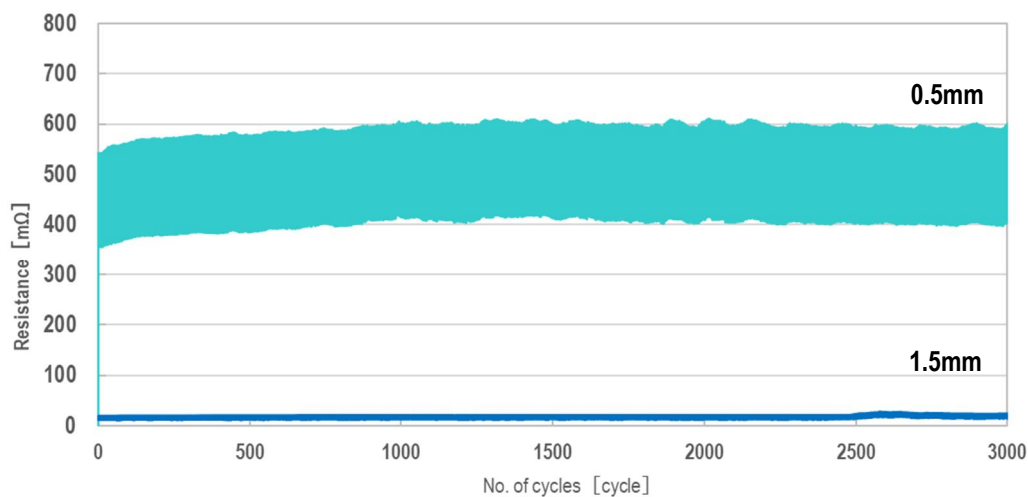
Graph 7. Monitoring result of thermal shock resistance
