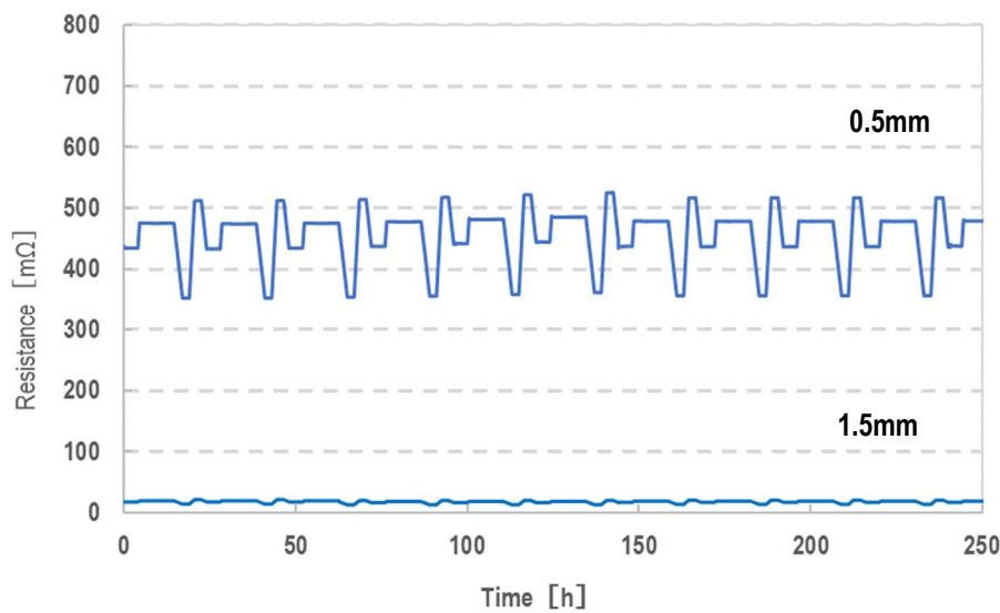
Graph 8. Monitoring result of temperature/humidity cycle resistance
