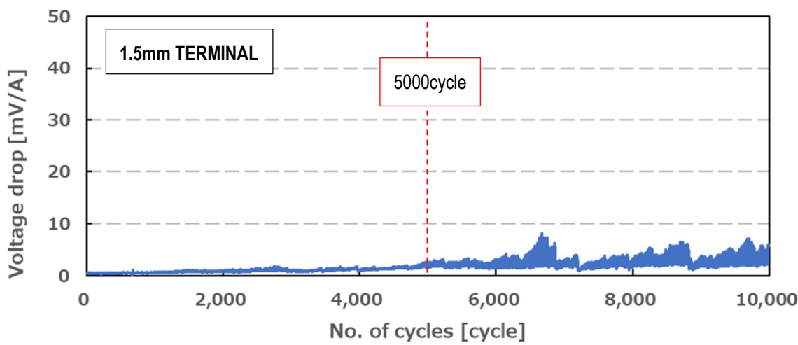
Graph 6. Monitoring result of 1.5mm terminal resistance for fretting corrosion
