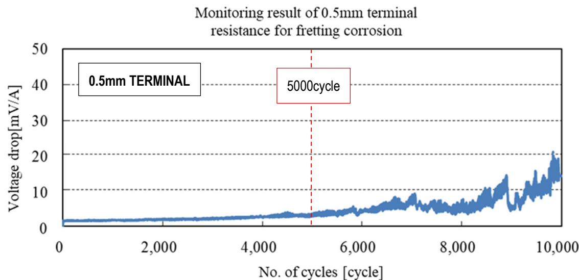
Graph 1. Monitoring result of 0.5mm terminal resistance for fretting corrosion
