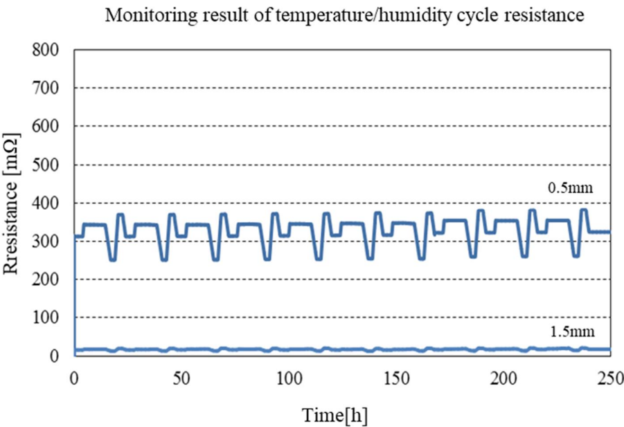
Graph 4. Monitoring result of temperature/humidity cycle resistance
