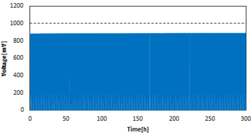
Graph3. Vibration with temperature change Resistance Monitor
