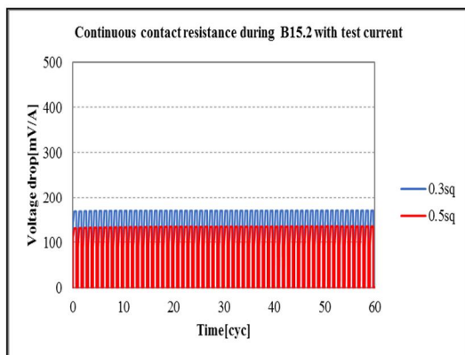
Graph 7. PG15 E14.0 Resistance Monitor
