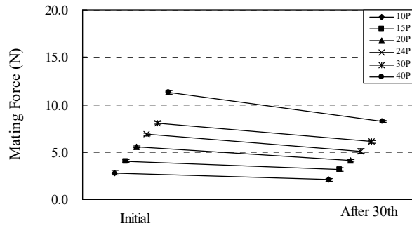
Graph.3 挿入力の変化：耐久性 A change of mating force: Durability
