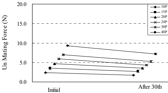
Graph.4 抜去力の変化：耐久性 A change of un mating force: Durability
