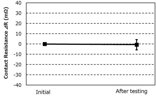
Graph8. A change of contact resistance (K Group : Humidity (Cycling))
