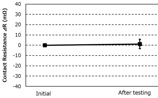
Graph7. A change of contact resistance (J Group : Humidity (Steady state))
