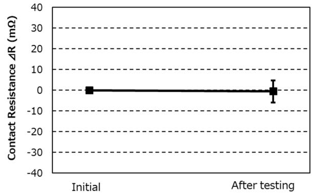
Graph10. A change of contact resistance (M Group : H 2 S gas)
