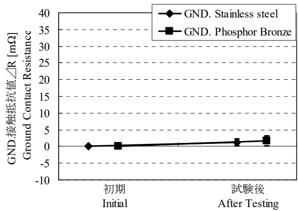
Graph 18. GND 接触抵抗値の変化 Hグループ: 塩水噴霧 A change of ground contact resistance H group : Salt Water Spray
