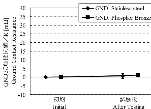
Graph 14. GND 接触抵抗値の変化 Fグループ:耐湿性(定常状態) A change of ground contact resistance F group : Humidity (Steady State)
