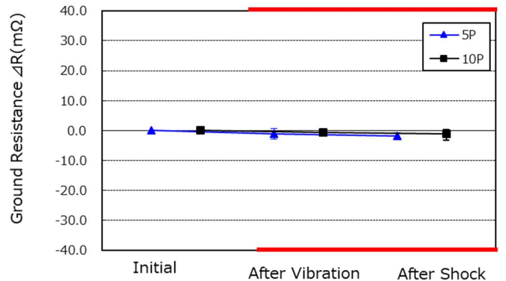
Graph.6 Vibration & Shock : Ground Resistance
