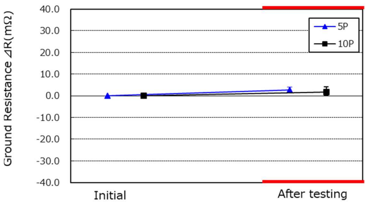
Graph.2 Durability : Ground Resistance
