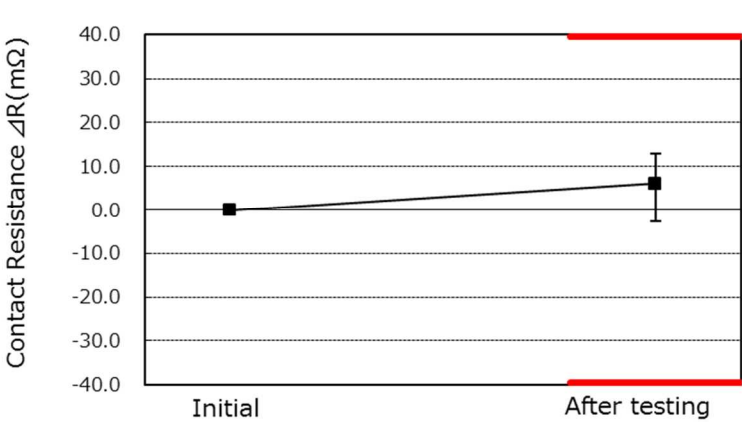
Graph.15 Salt Water Spray : Contact Resistance
