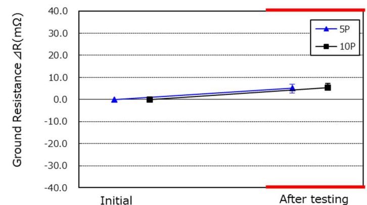
Graph.10 High temperature Life : Ground Resistance
