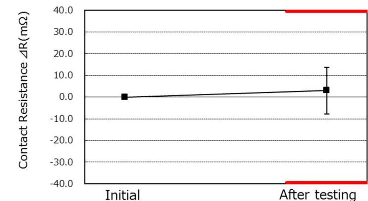
Graph.11 Humidity(Steady State) : Contact Resistance
