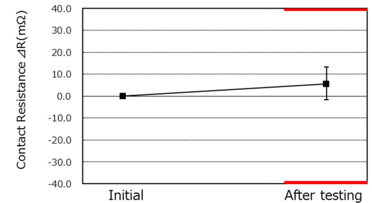
Graph.7 Thermal Shock : Contact Resistance
