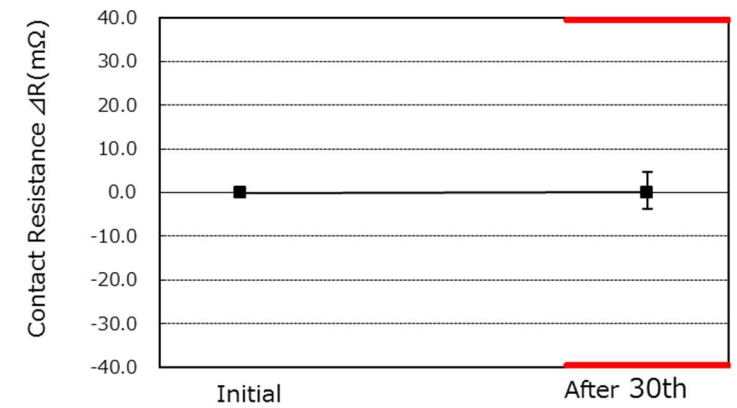
Graph.1 Durability : Contact Resistance
