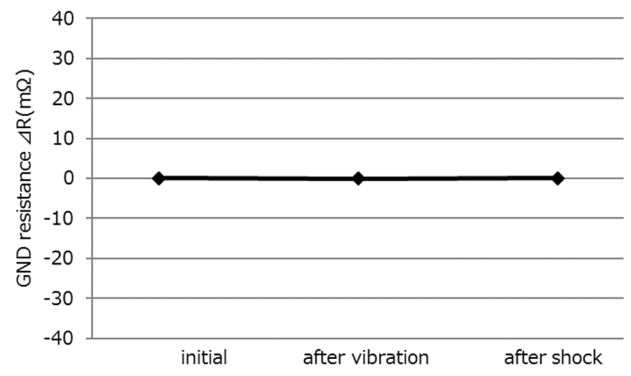
Graph 6. A change of GND resistance (D Group: Vibration/Shock)
