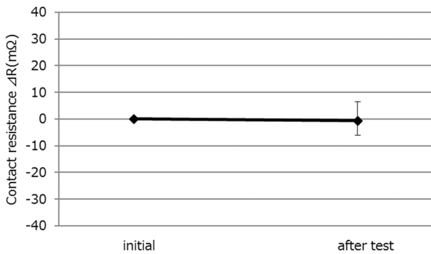
Graph 11. A change of contact resistance (F Group: Humidity(Steady state))
