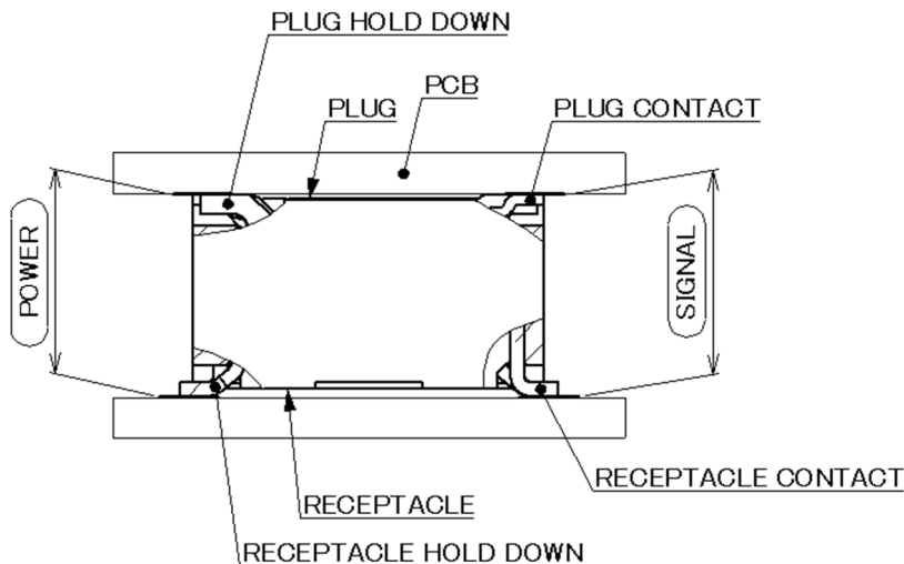
Fig.1 接触抵抗/Contact resistance
