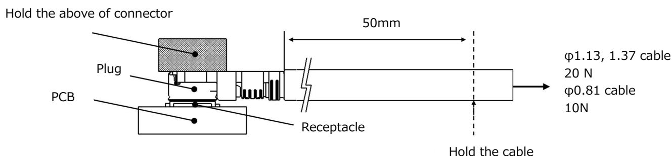
Fig. 4 Cable retention force at 0 degree
