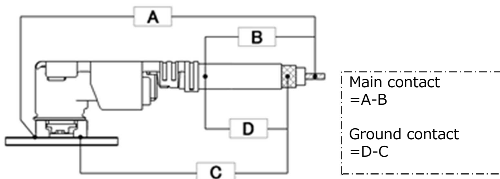
Fig. 1 Contact Resistance
