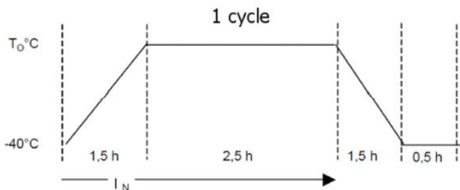
Fig 4. Temperature cycle
