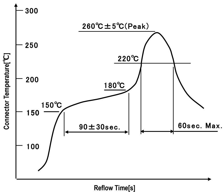
Fig 1.Reflow profile
