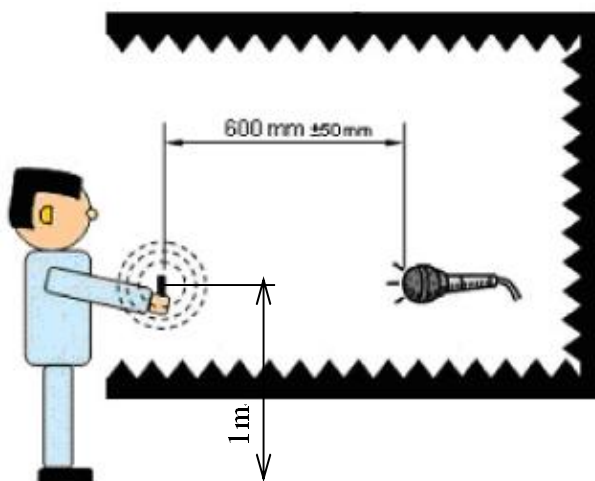
Figure 6. Locking noise
