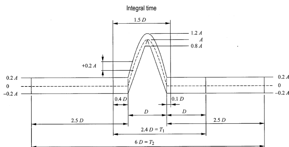
Fig.10.Sinusoidal half-wave
