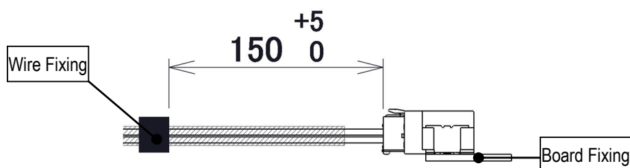
Fig.9. Fixing method
