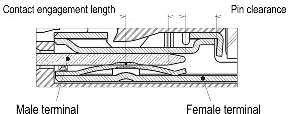
Fig 3. Contact engagement length, Pin clearance
