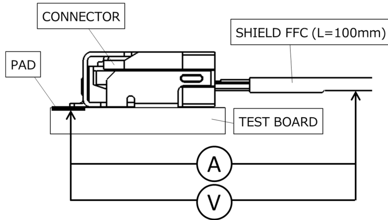
Fig.1 Contact Resistance
