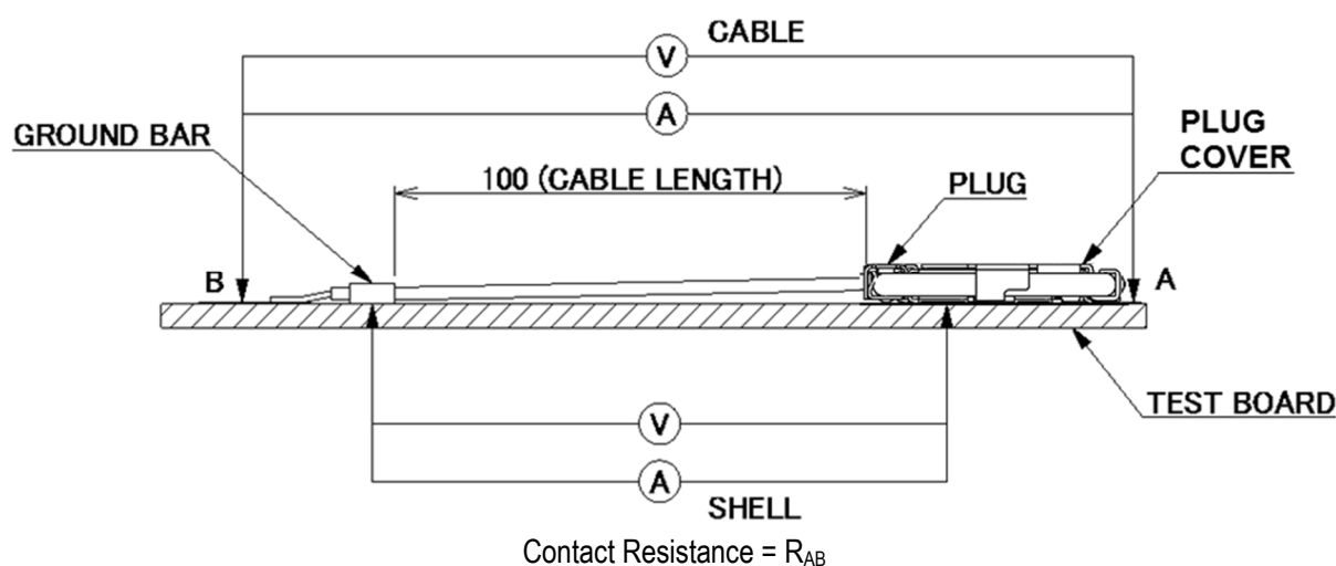
Figure 1. Contact Resistance
