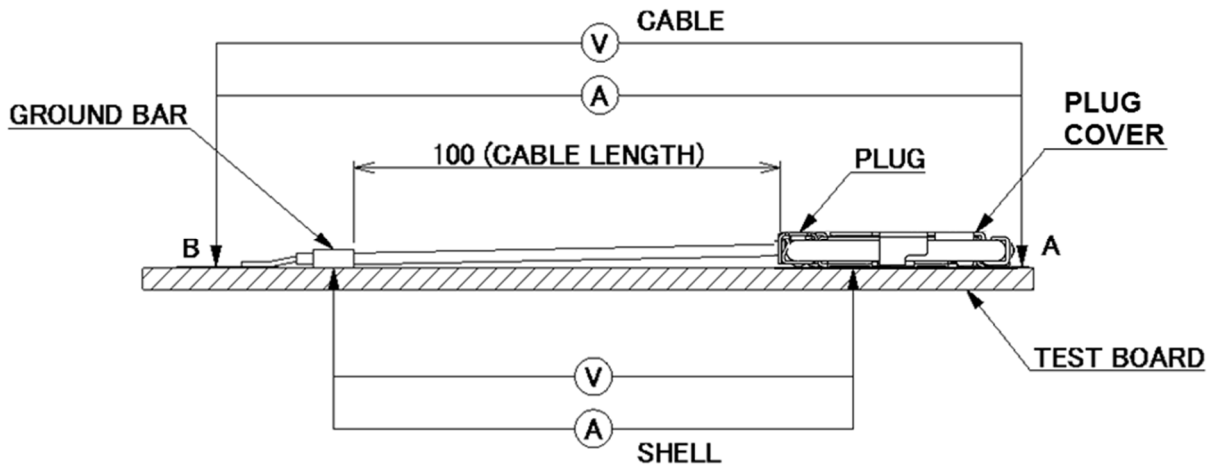
Fig.1 Contact Resistance
