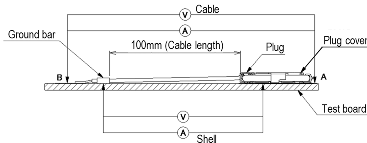
Figure 1. Contact Resistance
