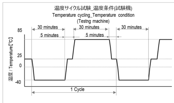
Fig.7 Temperature Transition time (Testing machine)
