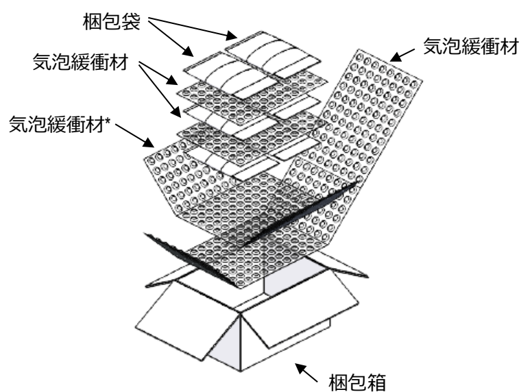
図 3. 梱包形態(ISH WIRE TO WIRE MALE HOUSING)
