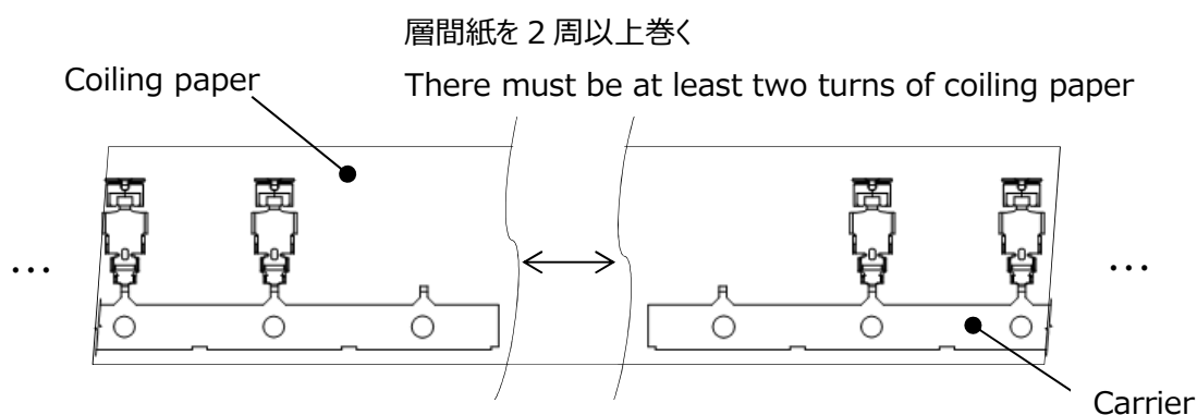
(Fig. 2) Connection of carrier
