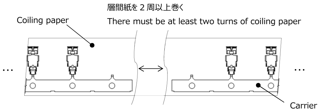
(Fig. 2) Connection of carrier
