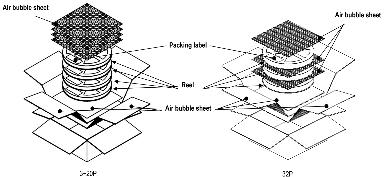
Fig2. Packing style
