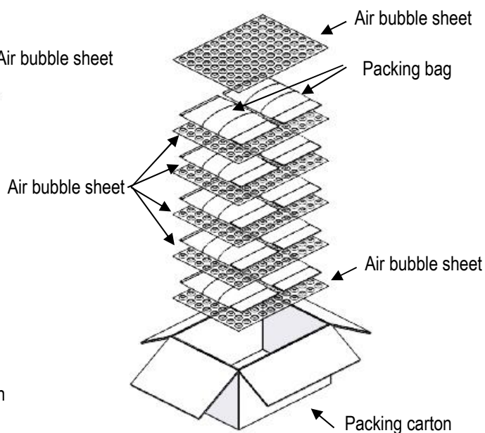
Fig.4. FEMALE RETAINER
