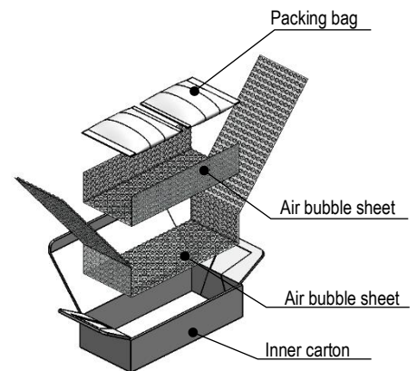
Fig3. Type of packing (Inner carton)
