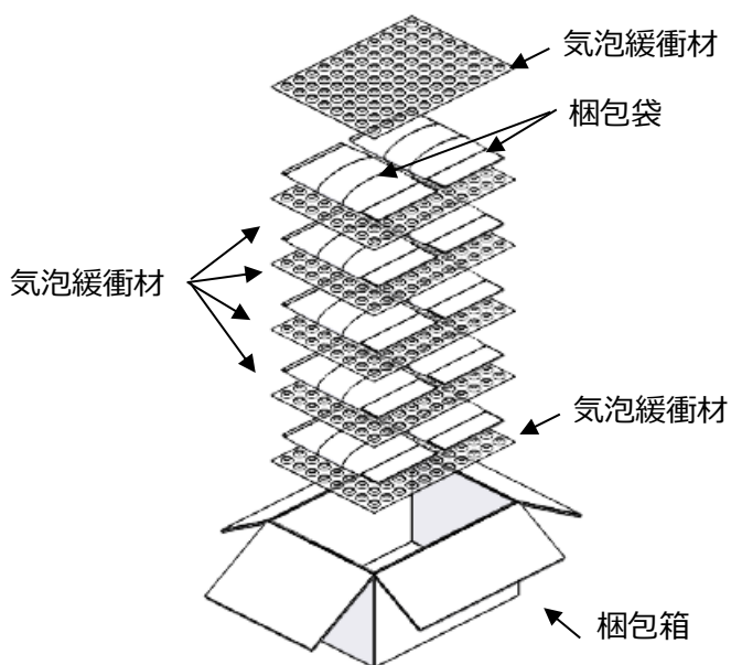
図 3. 梱包形態(FEMALE HOUSING REAR COVER)
