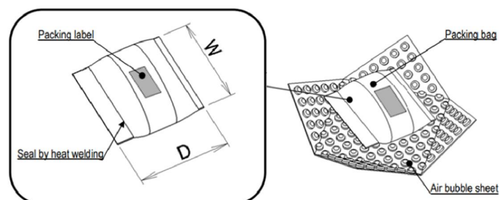
Fig2 Packing bag
