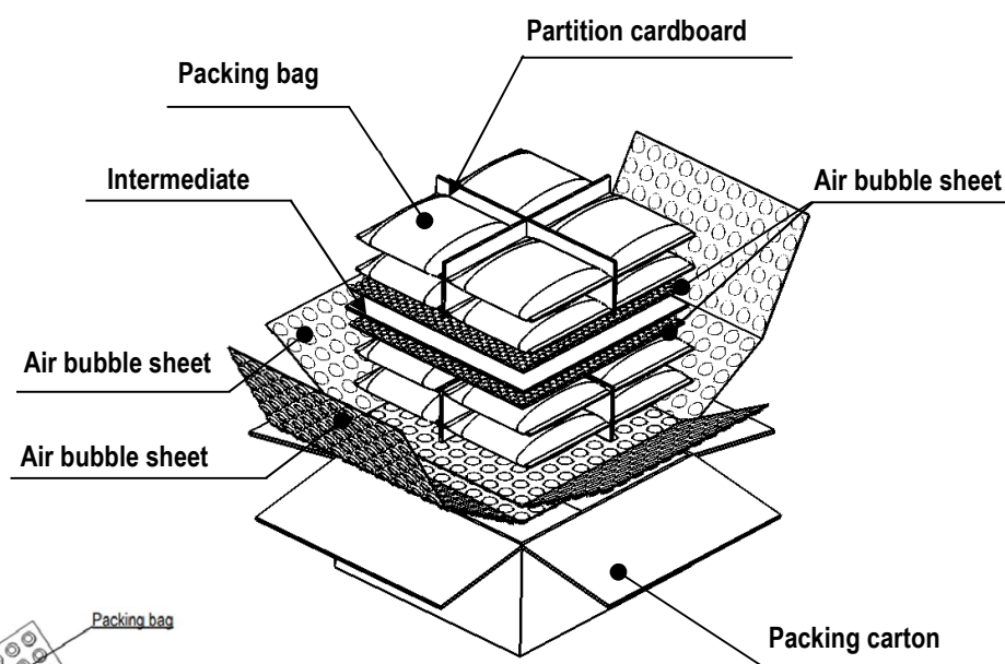
Fig3 Packing style
