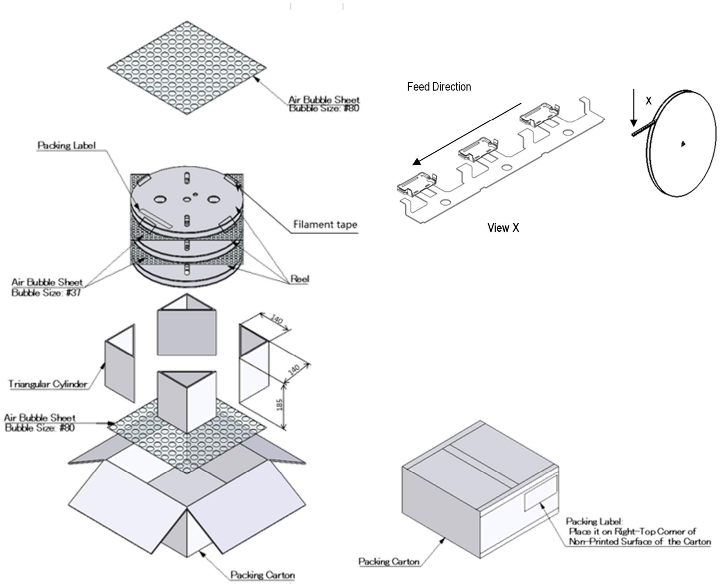
Fig.2 Packing Method
