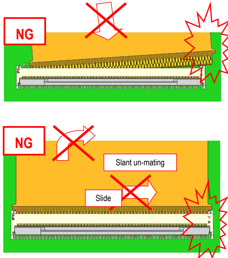
Fig.9 FPC insertion (NG)
