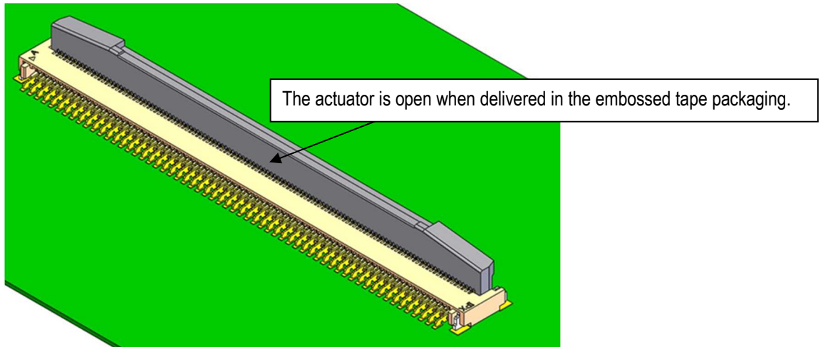
Fig.2 Connector mounting state
