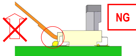
Fig.20 Flexion of FPC (NG)
