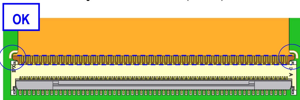
Fig.6 The check of FPC insertion (Reference)
