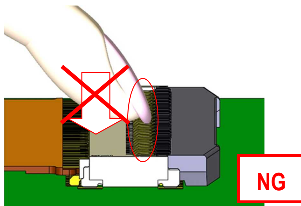
Fig.14 To lock actuator (NG)
