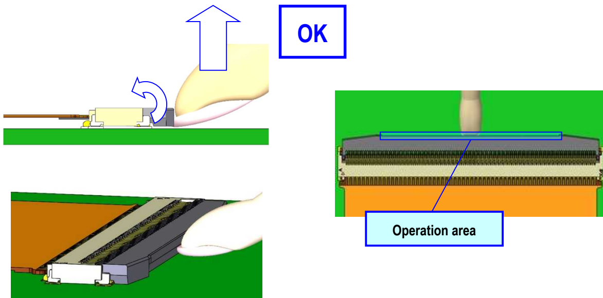
Fig.16 To release actuator (OK)
