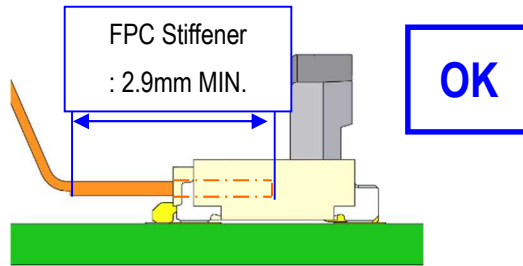
Fig.19 Flexion of FPC (OK)
