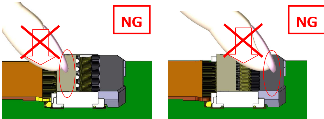
Fig.15 To lock actuator (NG)
