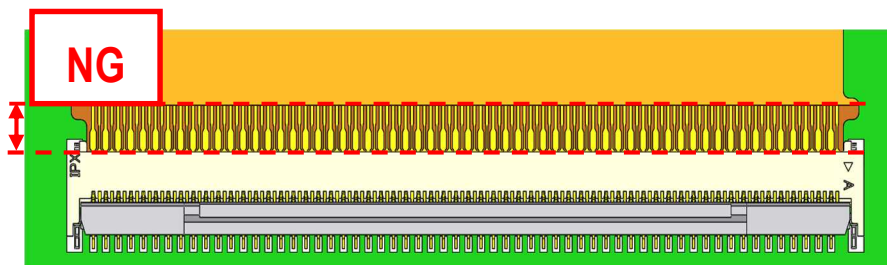
NG-① : Short insertion
