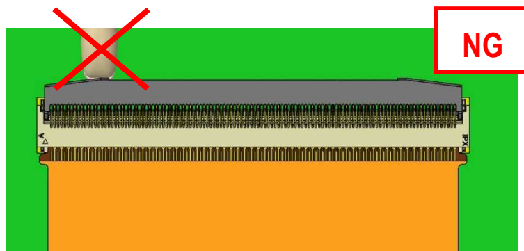
Fig.18 To release actuator (NG)
