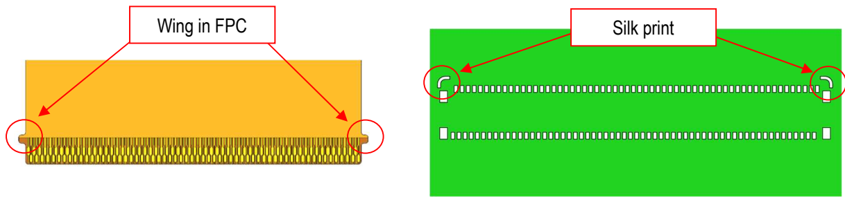
Fig.6 The check of FPC insertion (Reference)
