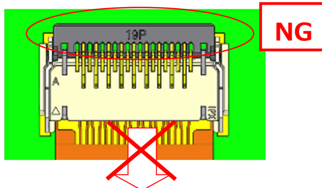
図 20. FPC の抜去方法 (NG) / Fig.20 To withdraw FPC (NG)
