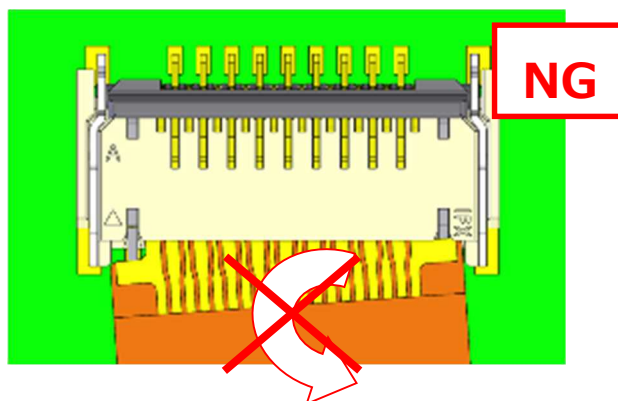
図 19. FPC の抜去方法 (NG) / Fig.19 To withdraw FPC (NG)
