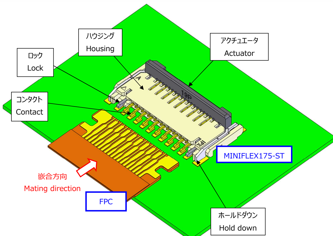
図 1. コネクタ各部名称 / Fig.1 Names of each part of the connector
