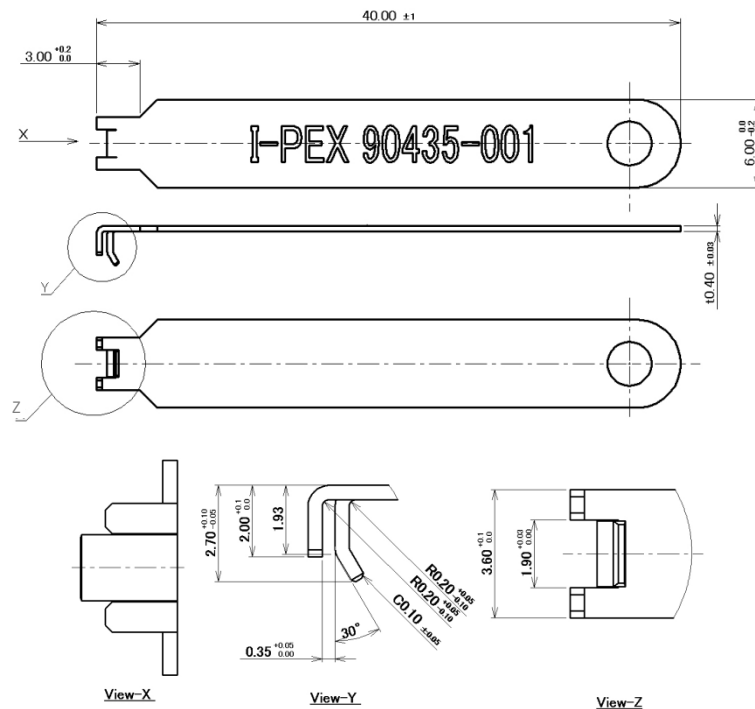
Fig. 1 推奨 挿抜 JIG (Part No. 90435-001)
