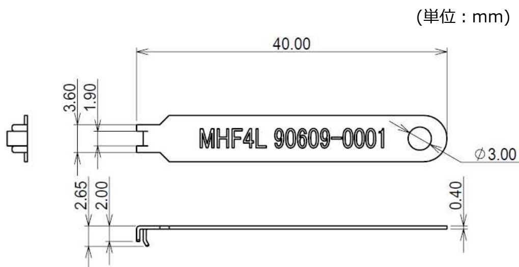
(Fig. 1) 推奨 抜去 JIG
