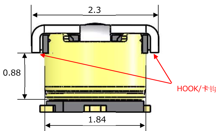
(Fig. 2) 抜去 JIG 引っ掛け形状配置図 (PLUG connector design feature to hook pull jig) (拔取治具的形状示意图)
