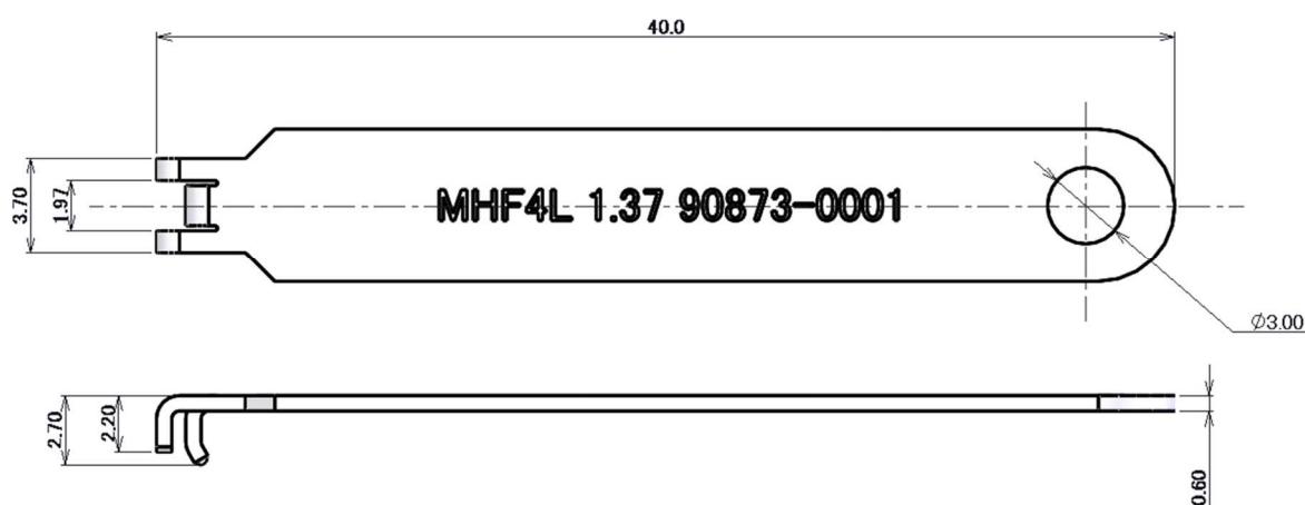
(Fig. 1) 推奨 抜去 JIG (Recommendation: Pushing & Pulling JIG) (推荐的拔取治具)
