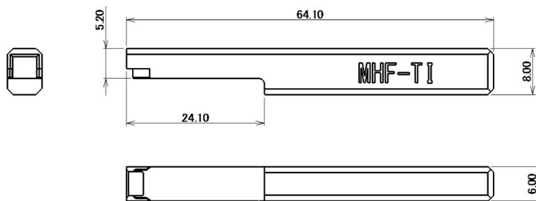
Fig. 7 MHF-TI 抜去 JIG
