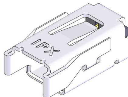
Fig. 2 MHF-TI RECEPTACLE
