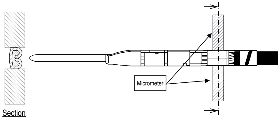
Fig 7. Wire barrel Crimp width measurement
