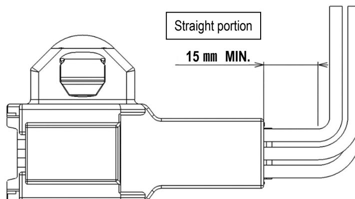
Fig 42. Arrangement of harnesses
