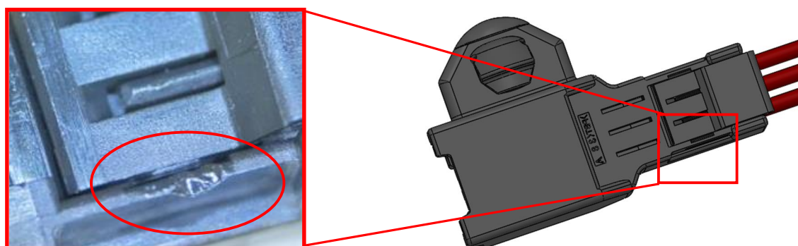
Fig.29. Example of damage on the secondary lock part
