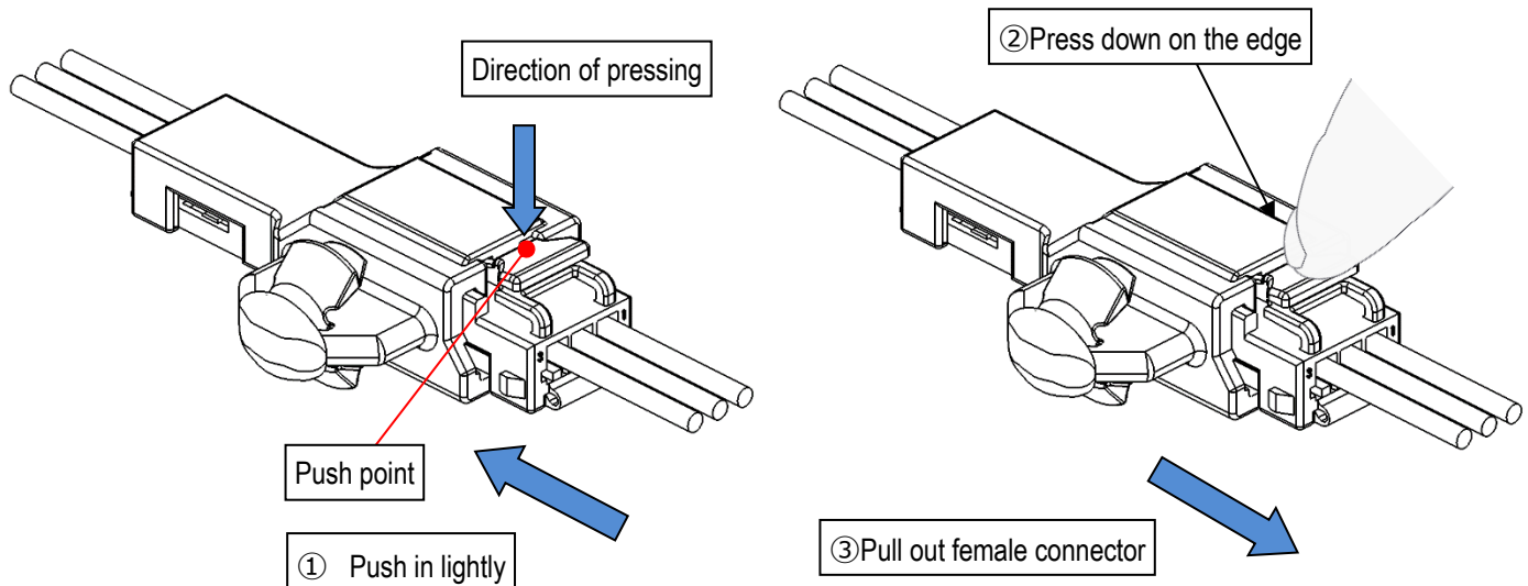
Fig39. Lock arm
