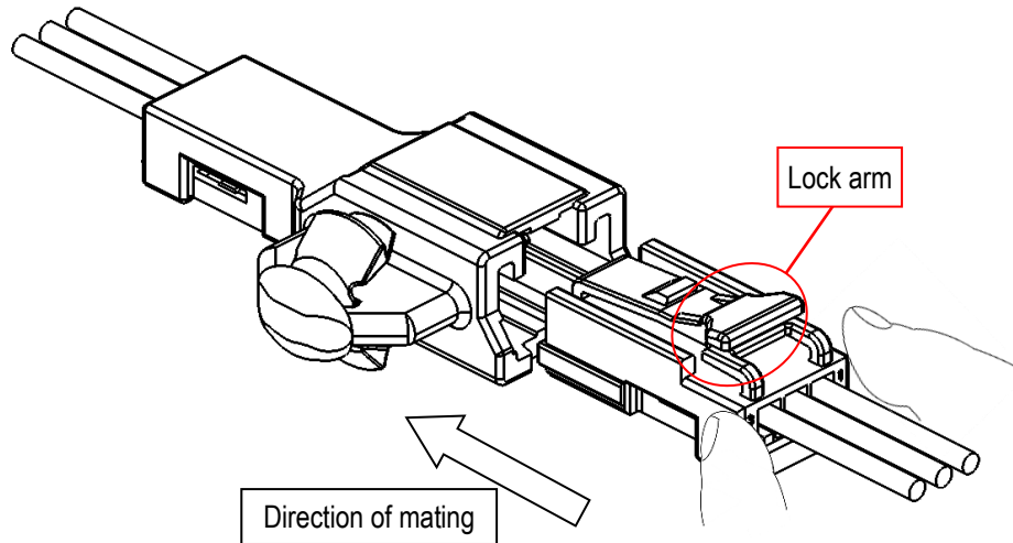
Fig37.Direction of mating
