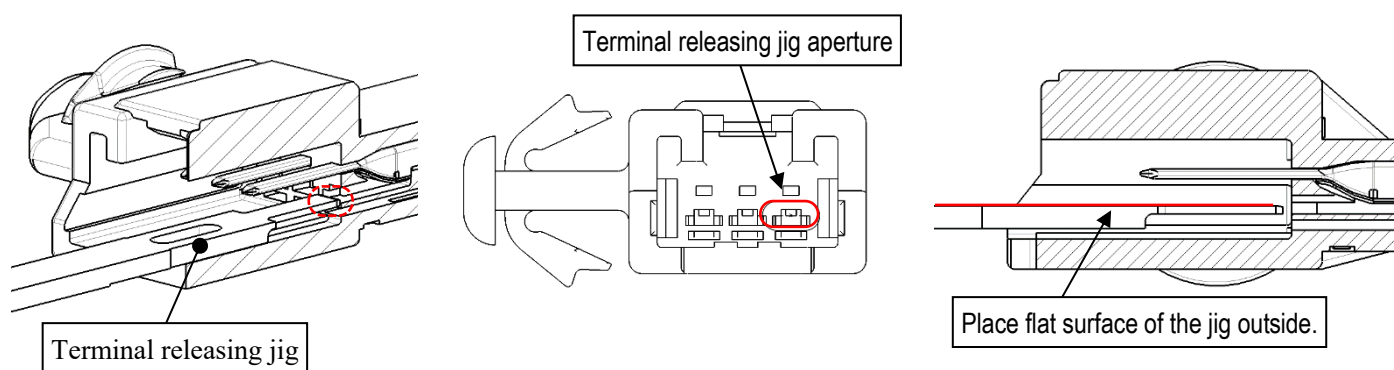
Fig 31. Female housing and Direction of release
