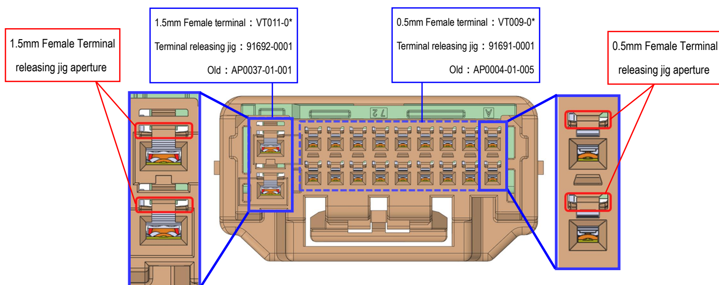
Fig 32. Releasing apertures location
