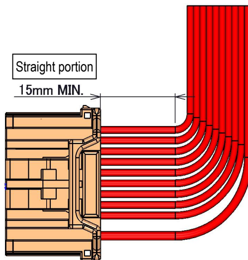
Fig 45. Arrangement of wires
