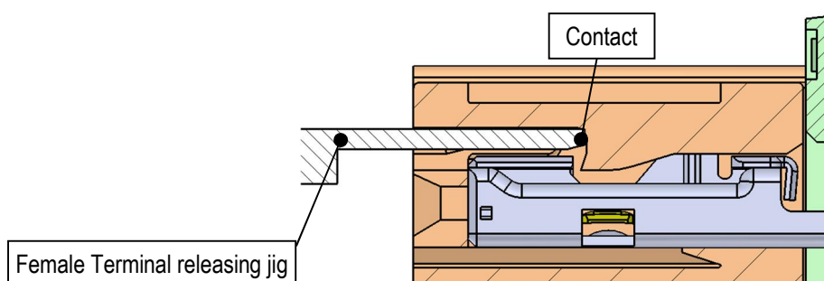
Fig33. Correct orientation of the releasing jig and the housing lance
