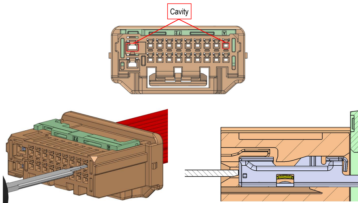
Fig 37. Incorrect insertion of the releasing jig
