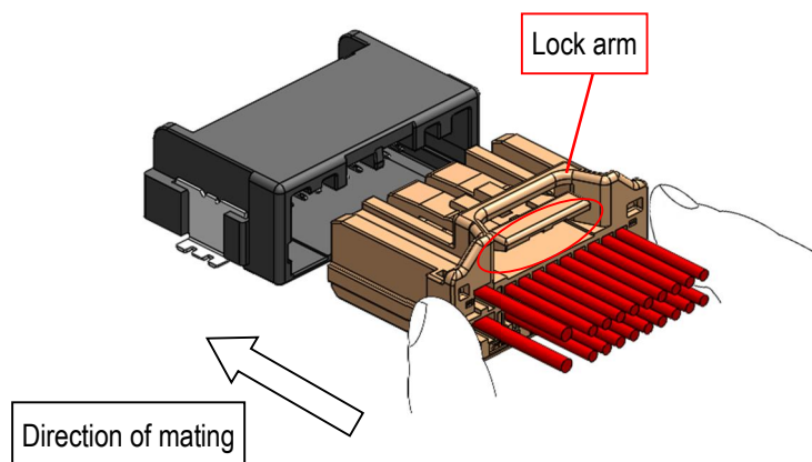
Fig 40. Direction of mating
