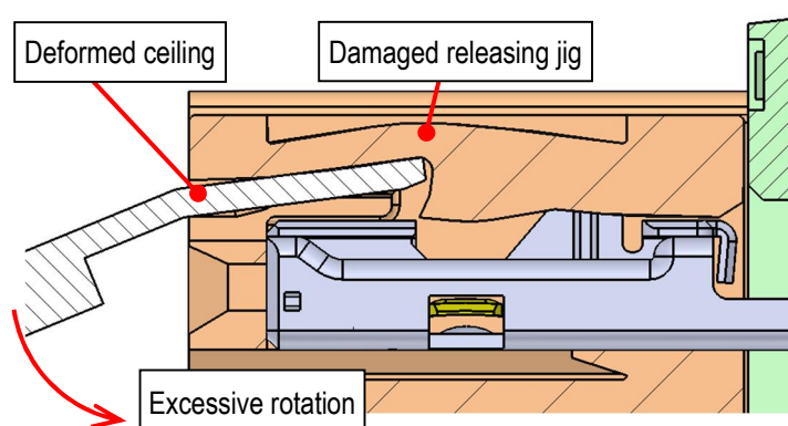
Fig36. Deformed ceiling, Damaged releasing jig
