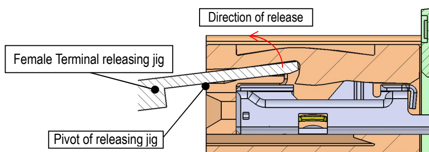
Fig34. Female Terminal releasing jig in operation
