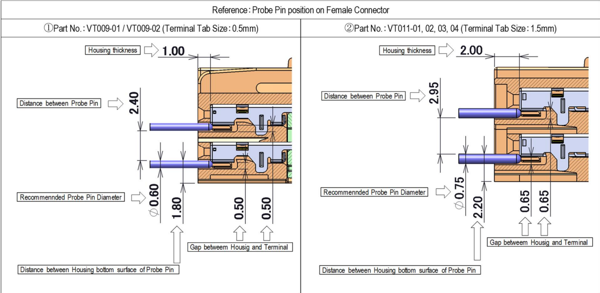
Fig 44. Conductivity test for female terminals (contacts)
