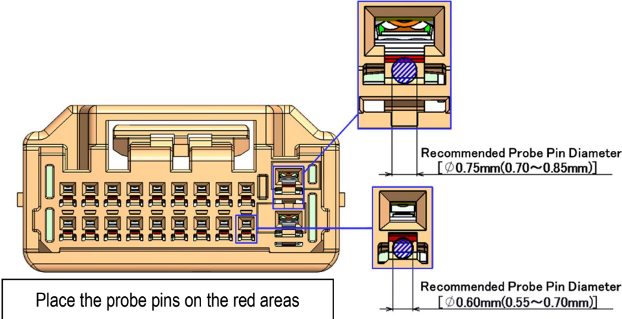
Fig 44. Conductivity test for female terminals (contacts)
