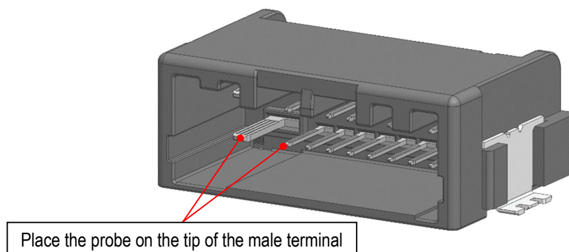
Fig 43. Conductivity test for male terminals (contacts)
